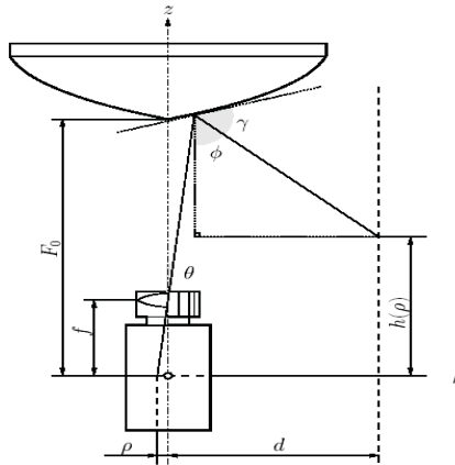
Fig. 8. Schematic diagram of the omni vision sensor
