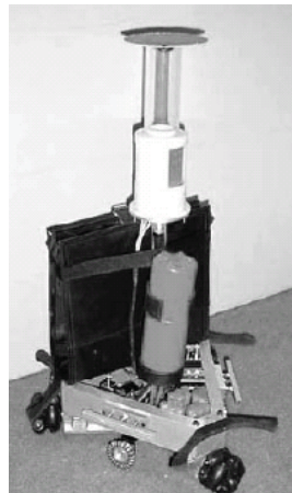
Fig. 1. A comprehensive omni directional robot having omni directional vision, motion and kicking systems
