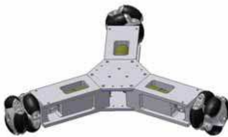
Fig. 4. (a) Three black omni directional poly-roller wheels act as actuators, (b) three free omni directional small-roller wheels used in a feedback mechanism
