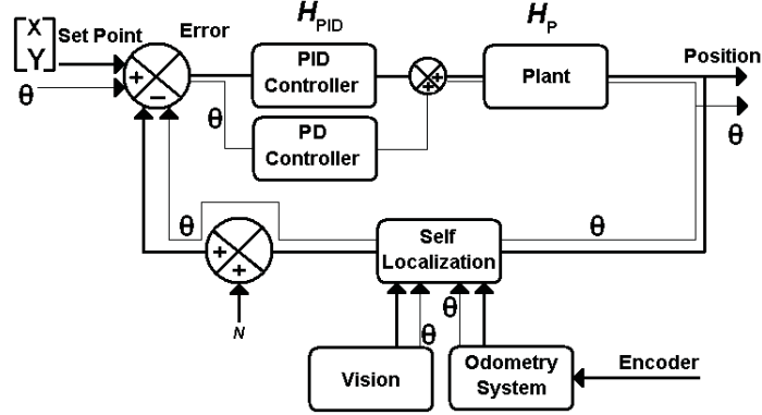
Fig. 6. Control diagram of the omni directional robot
