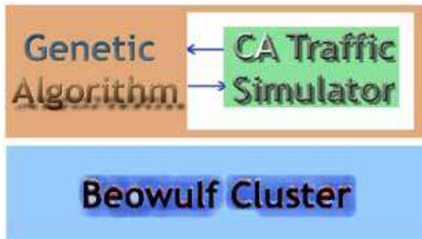
Fig. 1. Model Architecture
