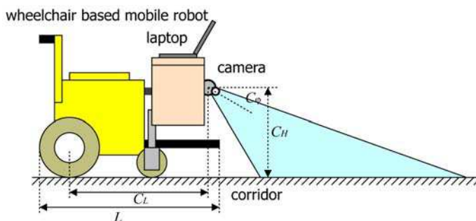
Fig. 1. Overview of mobile robot.
