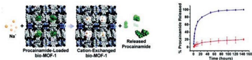
Figure 2. (Left) Scheme depicting cation-triggered procainamide release from Bio-MOF-1; (right) procainamide release profiles from Bio-MOF-1 (blue—PBS buffer; red—de-ionised nanopure water) (image from An et al. [30]—Copyright © 2009, American Chemical Society).
