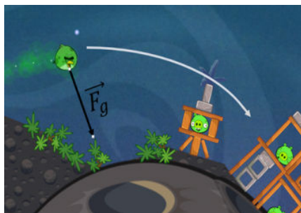
Figure 6. We can see that the force of gravity is pointing in the center of the small planet's mass, therefore also affecting the path of the bird's movement, which would circle for longer time if the force of gravity would be smaller or the velocity of the bird would be higher.
