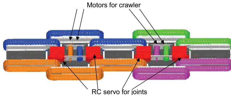
Fig. 11. The driving structure (Color indicates driving relationship between motors and crawlers)
