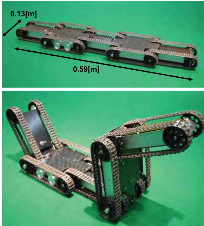
Fig. 10. Prototype of connected crawler robot
