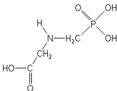
Figure 1. Molecular structure of N-(phosphonomethyl) glycine
