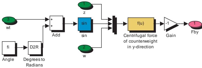
Figure 9. Calculation of centrifugal force F_{by} for the balancing mass
