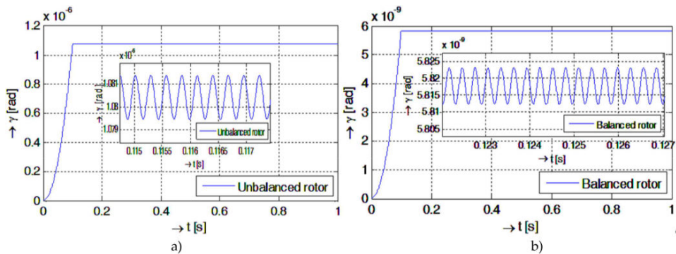
Figure 29. Complex twist angle with detail of the time course of: a) the unbalanced shaft, b) the balanced one
