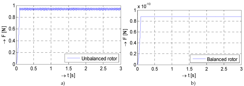
Figure 19. Force acting on bearings: a) prior to and b) after the rotor balancing
