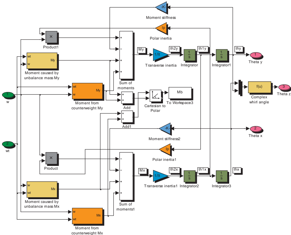
Figure 11. Subsystem Dynamic balancing
