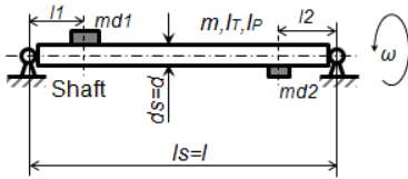
Figure 1. Parameters of rotating bodies: rotor and shaft
