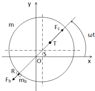
Figure 2. Analysis of forces in an unbalanced rotor
