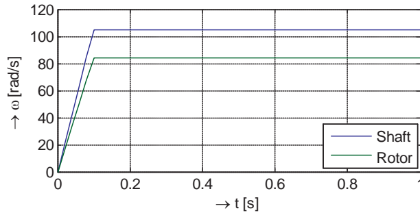
Figure 16. The graph showing angular speed course at starting of the rotor and shaft. In time of 0.1 s they reach the operating speed.
