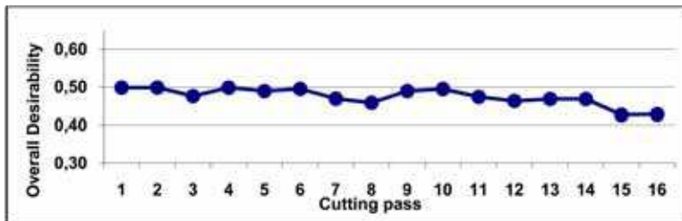
Fig. 8. Overall desirability function along cutting tool life-cycle. Parameter optimization based on handbooks. V_c=200 m/min; fz=0.08 mm; ap=0.4 mm
