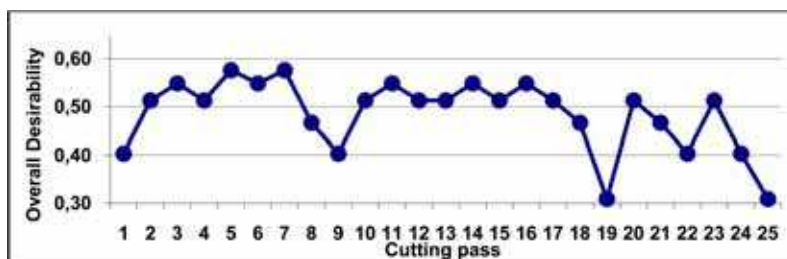
Fig. 10. Overall desirability function along cutting tool life-cycle. Parameter optimization based on RMSO. Vc=164m/min; fz=0.12mm; ap=0.4mm.
