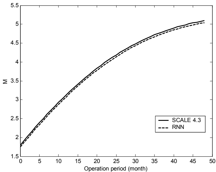
Figure 9. Change in M with respect to time in the blanket using Li_{20}Sn_{80} obtained by Scale 4.3 (Übeyli & Acir, 2007) and RNN
