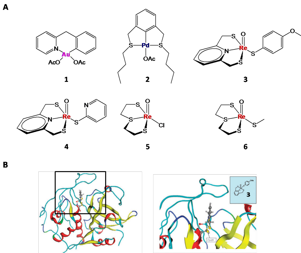
Figure 5. A) Structures of metal complexes with antileishmanial activity via inhibition of parasite cysteine proteases: (1) diaceto [2-[(2-pyridinyl- \kappa N)methyl] phenyl- \kappa C] gold(I), (2) aceto [2,6-bis [(butylthio- \kappa S)methyl]-phenyl- \kappa C] palladium(II), (3) ( p -methoxyphenylthiolato- \kappa S) [2,6-bis[(mercapto- \kappa S)methyl] pyridine- \kappa N 1 ] oxorhenium(V), (4) (2(1 H )-pyridinethionato- \kappa S 2 )[2,6-bis [(mercapto- \kappa S)-methyl] pyridine- \kappa N 1 ] oxorhenium(V), (5) chloro [2,2'-(thio- \kappa S)bis [ethanethiolato- \kappa S]] oxorhenium(V), (6) (methanethiolato) [2,2'-(thio- \kappa S)bis [ethanethiolato- \kappa S]] oxorhenium(V). B) Hypothetical model of oxorhenium(V) complex 3 binding to the active site cysteine of cathepsin B. Adapted from Ref. [25].
