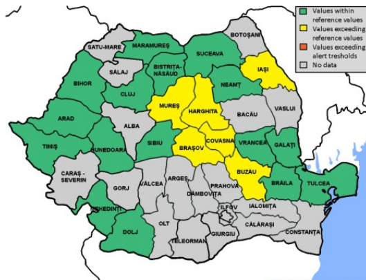
Figure 6. Nickel levels in soil in rural areas
