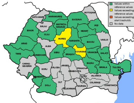
Figure 8. Manganese levels in soil in rural areas
