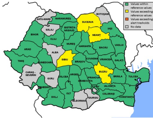
Figure 13. Zinc levels in soil in urban areas
