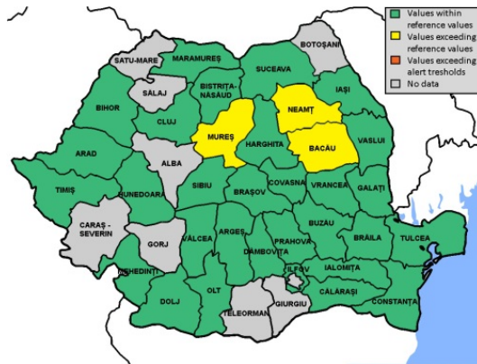
Figure 14. Zinc levels in soil in rural areas
