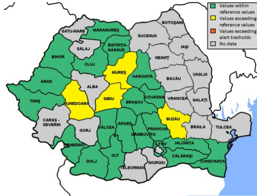
Figure 17. Arsenic levels in soil in urban areas
