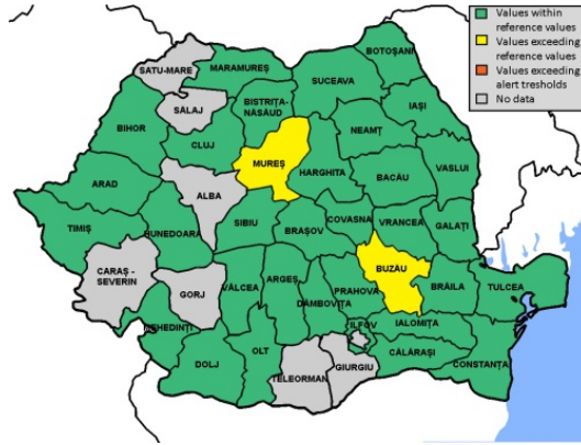
Figure 9. Total chromium levels in soil in urban areas
