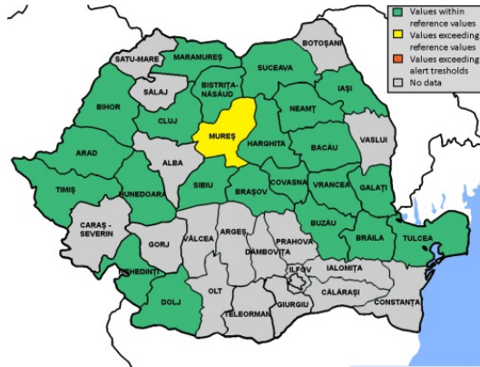
Figure 7. Manganese levels in soil in urban areas
