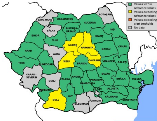
Figure 10. Total chromium levels in soil in rural areas
