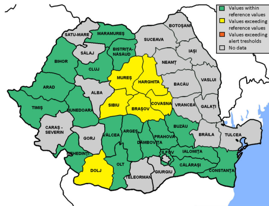
Figure 18. Arsenic levels in soil in rural areas
