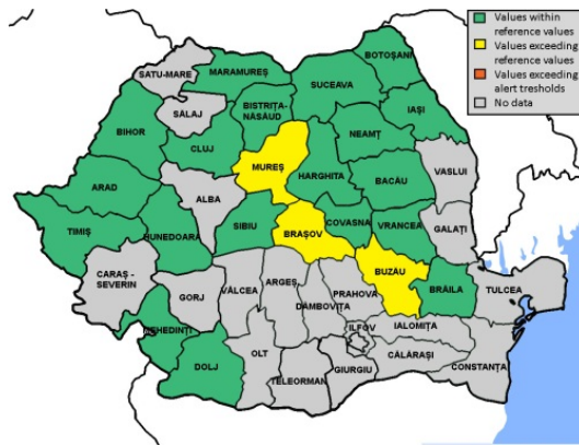
Figure 5. Nickel levels in soil in urban areas
