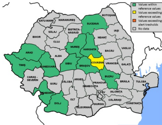
Figure 12. Total cobalt levels in soil in rural areas
