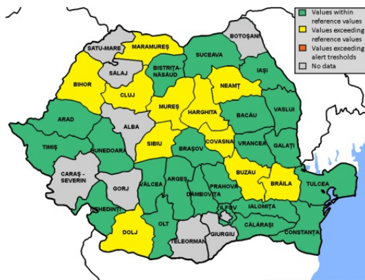
Figure 4. Copper levels in soil in rural areas
