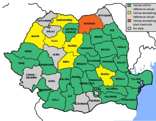
Figure 3. Copper levels in soil in urban areas
