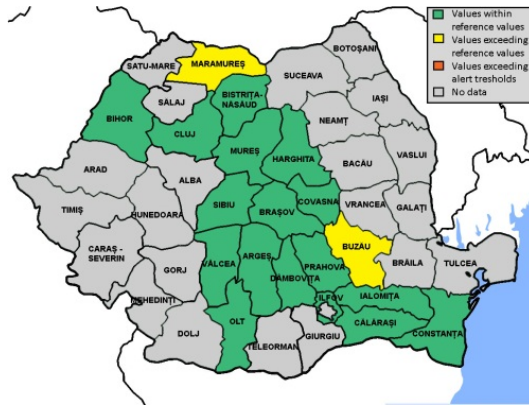
Figure 15. Mercury levels in soil in urban areas
