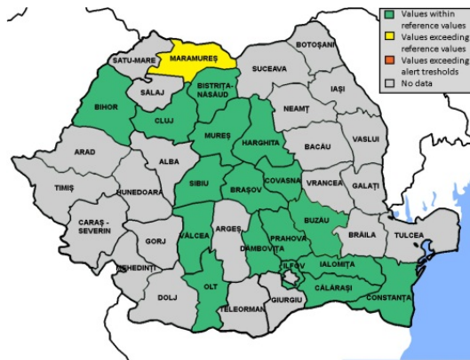
Figure 16. Mercury levels in soil in rural areas
