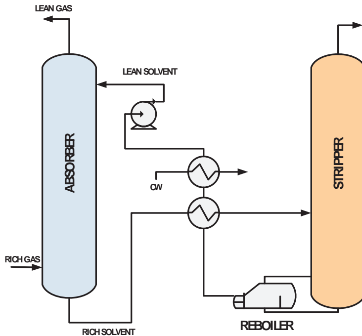
Figure 6. CO 2 capture by chemical absorption
