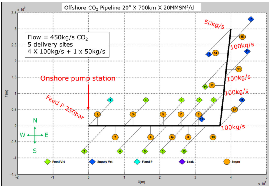
Figure 16. Hypothetical 20" X 700 km sub-sea pipeline for 20MMSm 3 /d of liquid CO 2 (≈450kg/s) at 250 bar from onshore plant to five offshore EOR wellheads (4X100kg/s + 1X50kg/s) 2100m deep, 380km from the coast.
