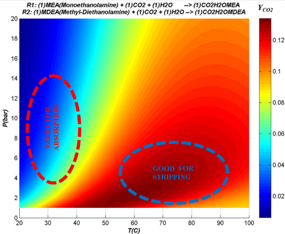
Figure 15. Equilibrium vapor phase mol fraction of CO 2 ( Y_{CO_2} ) versus T(^{\circ}C) \times P (bar) under reactive VLE: 1 mol of a 16.7%mol CO 2 natural gas is contacted with 1.2 mol of a liquid solvent with 14.5%mol MEA, 14.5%mol MDEA and 71%mol water.
