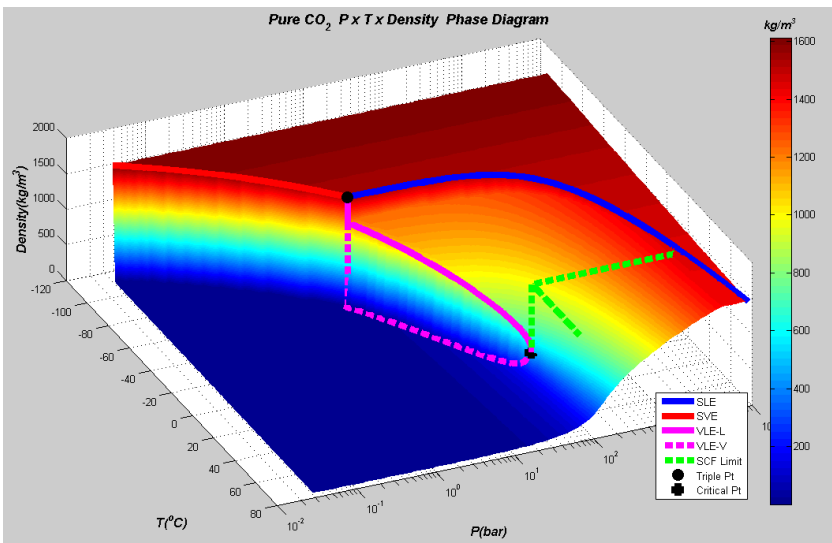
Figure 5. Density x Pressure x Temperature of Pure CO 2 [with TP and CP points, VLE, SVE & SLE lines and SCF domain]
