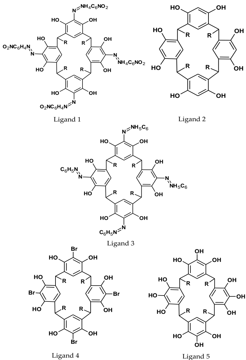
Figure 2. The structure of host molecules.
