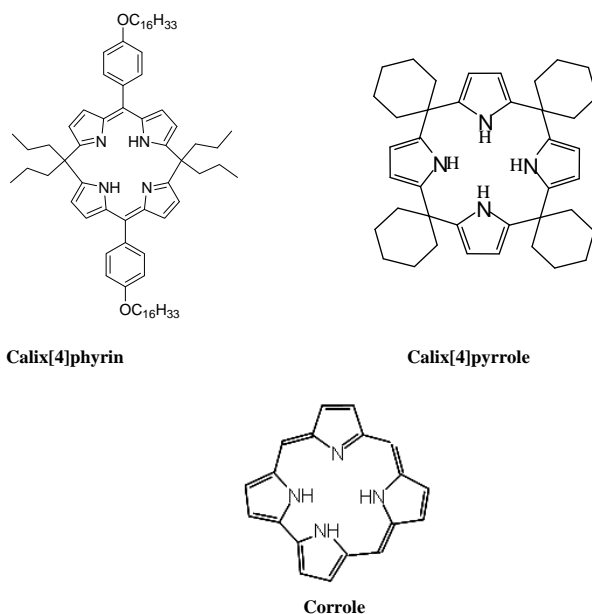
Figure 1. The structure of pyrrole hosts.
