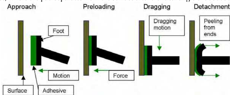
Figure 6. Idealised motion of a compliant robotic foot
