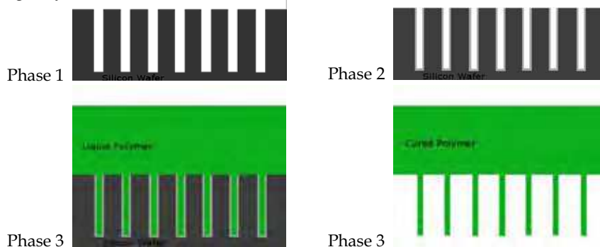
Figure 2. A polymeric micro-hair manufacture procedure
