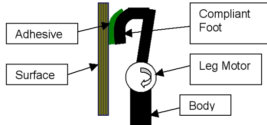
Figure 7. Foot Mechanism Design
