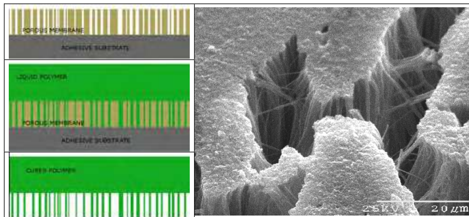
Figure 13. Nano moulding technique and Scanning Electron Microscope (SEM) image of the results
