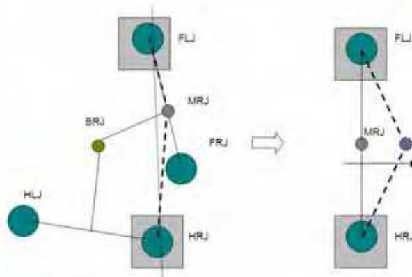
Figure 9. The RGR is represented in its unstable configuration the left; on the right is a schematic representation of the gecko robot, showing the model to be studied for the understanding of its unstable configuration. (FLJ=Fore Left Joint; HRJ=Hind Right Joint; FRJ=Fore Right Joint; HLJ=Hind Right Joint; BRJ=Back Right Joint; MRJ=Middle Revolute Joint.)
