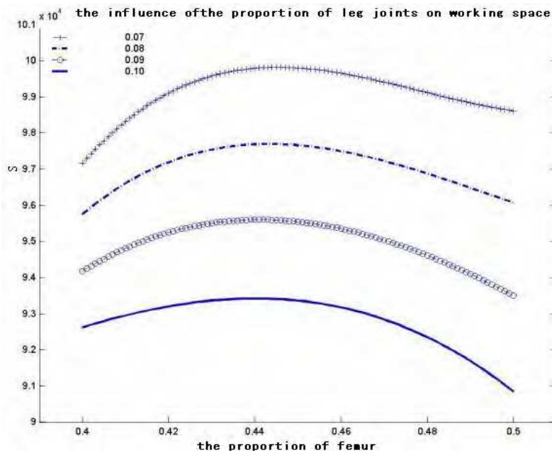
Figure 5. The influence of the proportion of leg joints on working space
