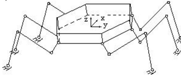
Figure 6. The simplified structure model of hexapod walking robot
