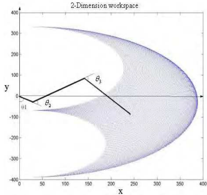
Figure 4. The “Cloudy graph” of foot tip working space
