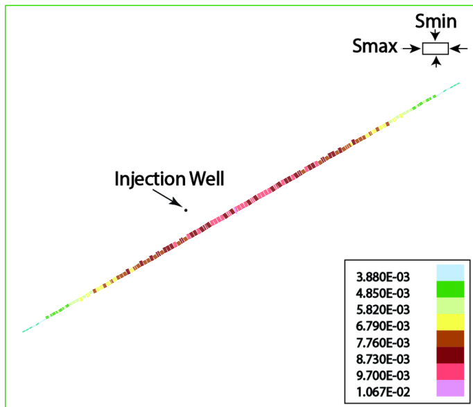
Figure 4. Fault shear displacement 2 ½ hours after shut-in.
