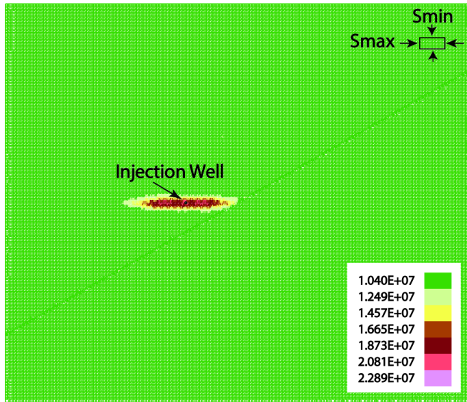
Figure 3. Pore pressure distribution 2 ½ hours after shut-in.
