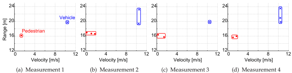
Figure 4. Sequence of range and velocity measurements.
