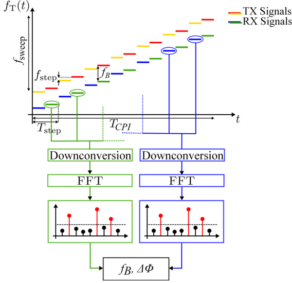
Figure 2. MFSK waveform principle with two intertwined transmit signals.
