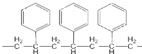
Figure 3. Molecular structure of polystyrene
