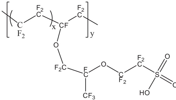
Figure 5. Molecular structure of Nafion
