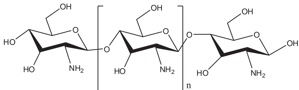
Figure 7. Molecular structure of chitosan
