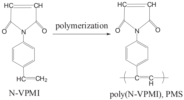
Scheme 1. Synthesis of polymaleimido-styrene
