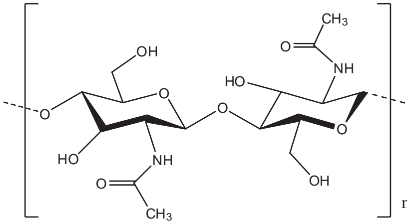
Figure 6. Molecular structure of chitin
