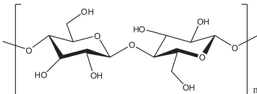
Figure 4. Molecular structure of cellulose
