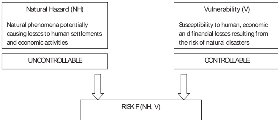
Figure 1. Natural Hazard, Vulnerability and Risk
