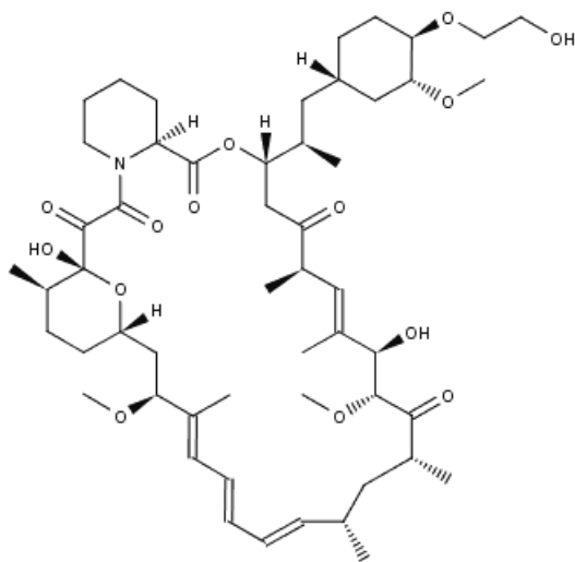
Figure 9. Chemical structure of everolimus.
