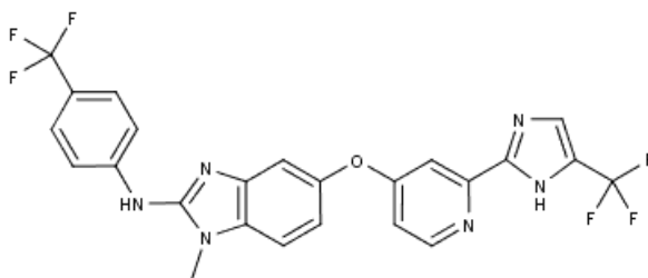
Figure 4. Chemical structure of RAF265.
