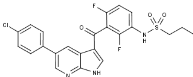
Figure 6. Chemical structure of vemurafenib.
