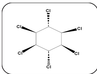
Figure 1. Chemical structure of hexachlorocyclohexane
