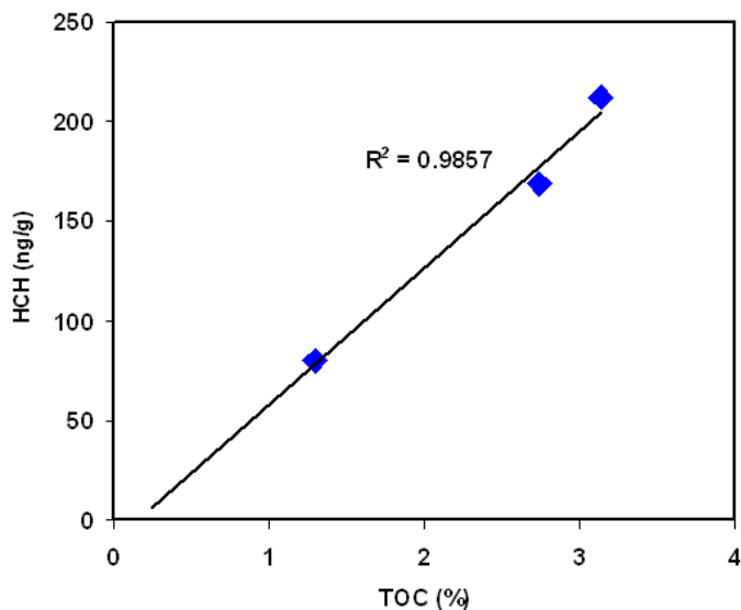
Figure 4. Correlation of HCH with TOC [Manko estuary]
