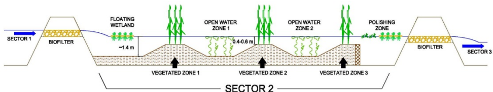
Figure 7. Scheme of the sequential model of wetland in sector 2 (longitudinal section)
