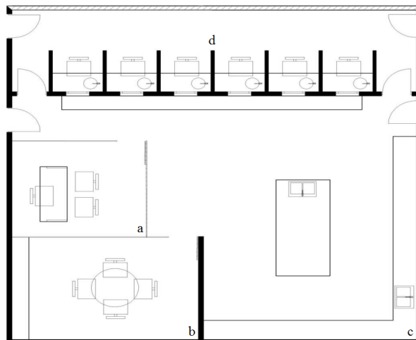
Figure 1. An example of layout of a sensorial analysis laboratory (Isaac et al., 2012a).
