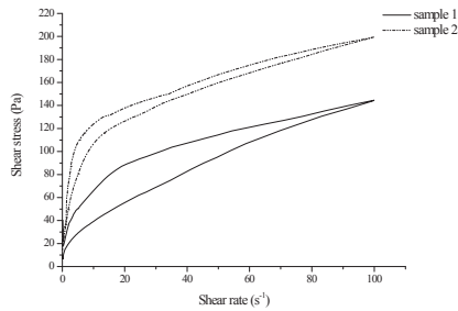
Figure 13. Comparison between flow curves of different samples.
