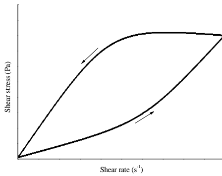
Figure 8. Flow curve of a thixotropic material.
