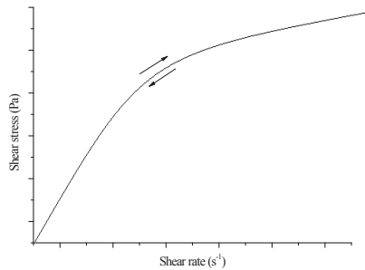
Figure 6. Flow curve of a pseudoplastic material.
