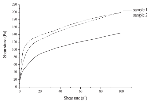
Figure 12. Comparison between flow curves of different samples (a thixotropic and a plastic fluid).
