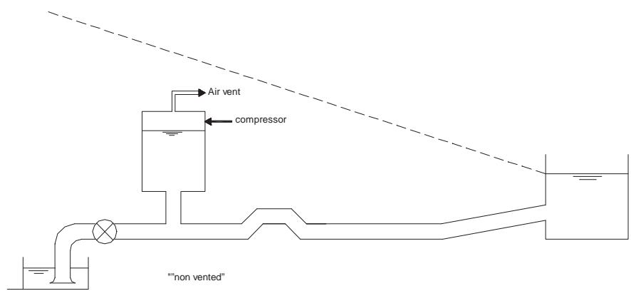
Figure 7. Non-aerated surge vessel
