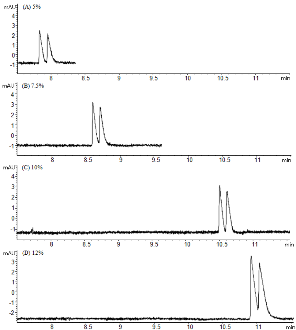
Figure 9. Effect of the concentration of tert-butanol on the separation of the enantiomers of Huperzine A: (A) 5%, (B) 7.5%, (C) 10% and (D) 12% (v/v). Separation conditions: BGE: 50 mM sodium acetate (pH 5.0), 0.2% (w/v) poly-LL-SUAV; pressure injection, 30 mbar for 3 s; applied voltage, 20 kV; temperature, 25 °C; fused-silica capillary, 64 cm (55.5 cm effective length) \times 50 \mu m i.d.; detection, 230 nm [55].
