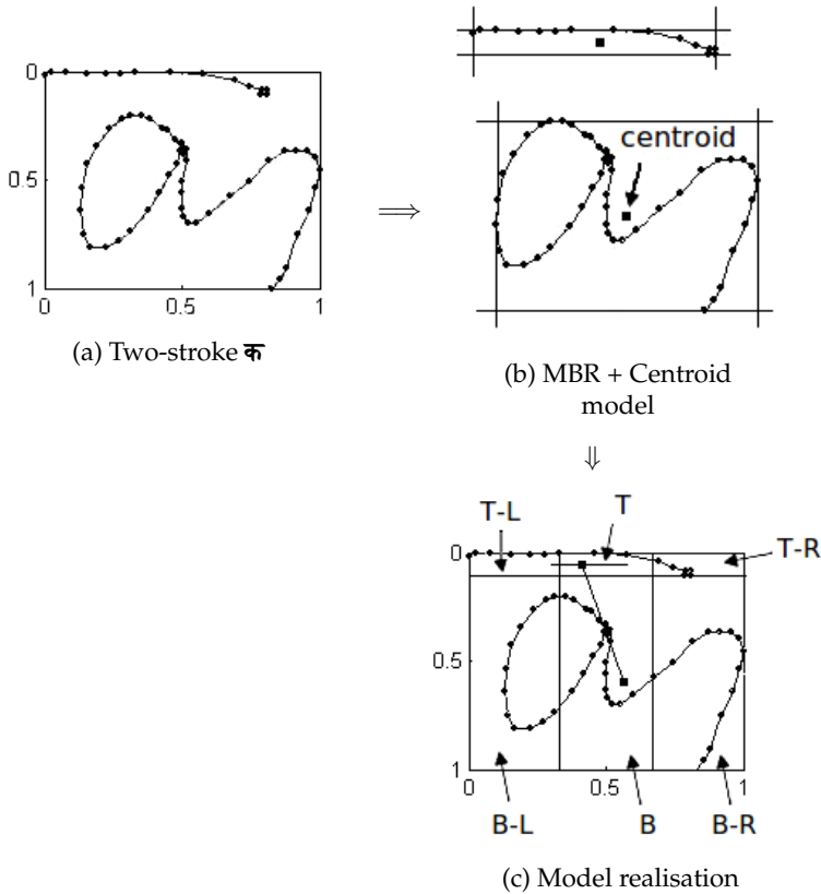
Figure 7. Pairwise spatial relation for a two-stroke क [40].
