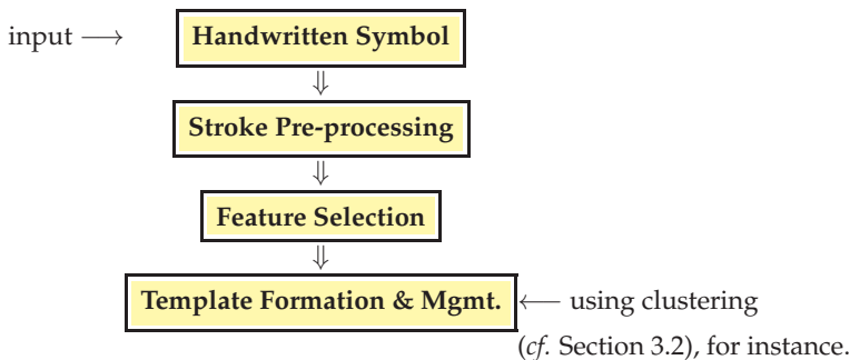
Figure 3. Learning strokes from the handwritten symbols. In this illustration, we present a basic concept to form template via clustering of features of the strokes immediately after they are pre-processed.
