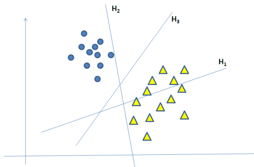
Figure 1. Separation hyperplanes. H_1 does not separate the two classes; H_2 separates but with a very tiny margin between the classes and H_3 separates the two classes with much better margin than H_2
