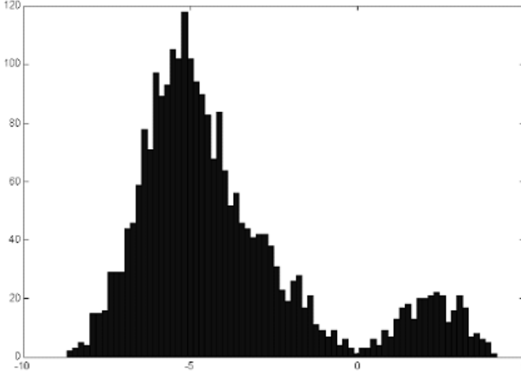
Figure 5. Output histogram of a binary one-against-all classifier
