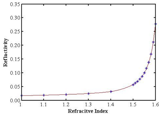
Figure 10. Reflectivity with refractive index of analyte[61]
