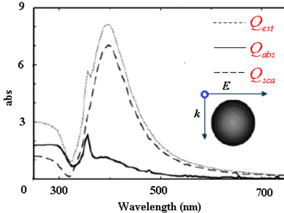
Figure 2. Optical coefficients for a silver nanosphere[23]
