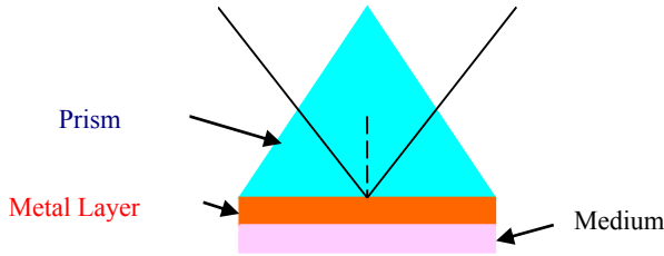
Figure 3. Kretschmann configuration
