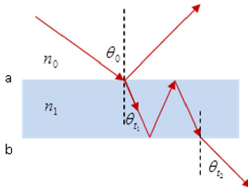
Figure 4. Reflection and refraction at the interface
