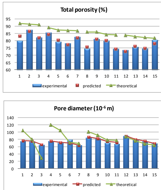
Figure 12. Results of nonwoven fabric porosity parameters
