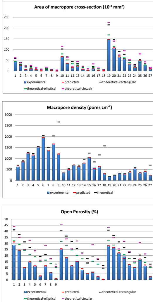
Figure 10. Results of woven fabric porosity parameters
