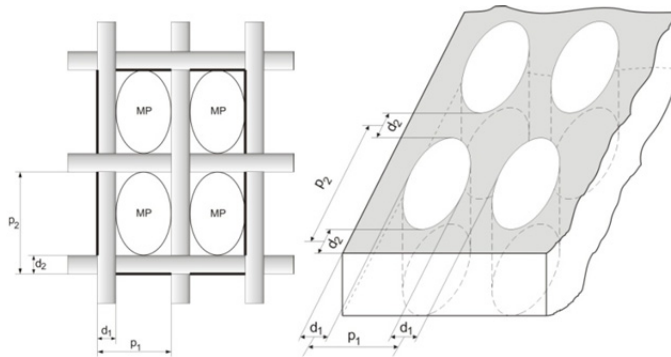
Figure 6. 2D and 3D presentations of an ideal model of the porous structure of a woven fabric [27, 28] (d – yarn thickness, p – yarn spacing, MP - macropore; 1, 2 indicates warp and weft yarns, respectively)
