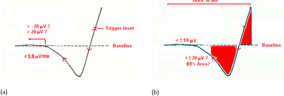
Figure 8. Description T2 and NM. In T2 (a), the MUAP onset is determined from the trigger to a point with slope < 0.8 \mu\text{V/ms} over a 1 ms. If there is a point before with amplitude > 20 \mu\text{V} , a new point fulfilling the slope criterion is looked for. In NM (b), the peak with maximum deviation from the BL is identified. The area of the MUAP from the first sample to the peak is calculated. Then the sample point with 90% of this area to the peak is obtained. If the absolute amplitude at this point is greater than 20 \mu\text{V} , a sample with 10 \mu\text{V} amplitude towards the beginning will be the MUAP onset. Otherwise a point toward the peak with 20 \mu\text{V} amplitude is reached. The MUAP onset then will be the point with amplitude 10 \mu\text{V} toward the first sample.
