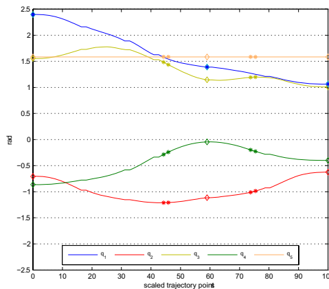
(b) 2 nd iteration of trajectory planning
