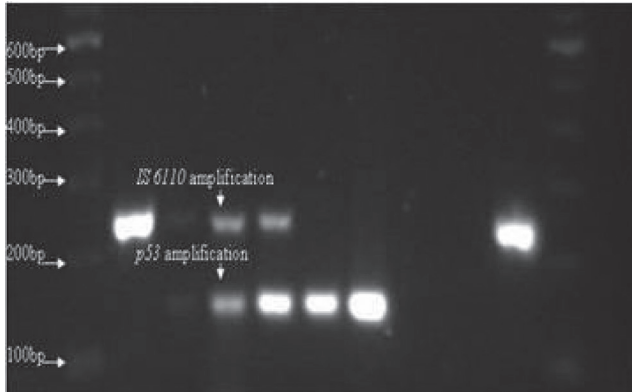
Figure 1. Agarose gel showing amplification of p53 and ISP6110. Amplifications were performed using marker 100 bp (M) and DNA from M. tuberculosis ATCC 27294 (P), various isolate (1-5), negative control, B. subtilis (N), positive control (PP).
