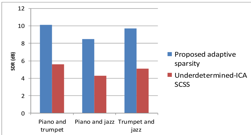
Fig. 11. Performance underdetermined-ICA SCSS method and proposed method
