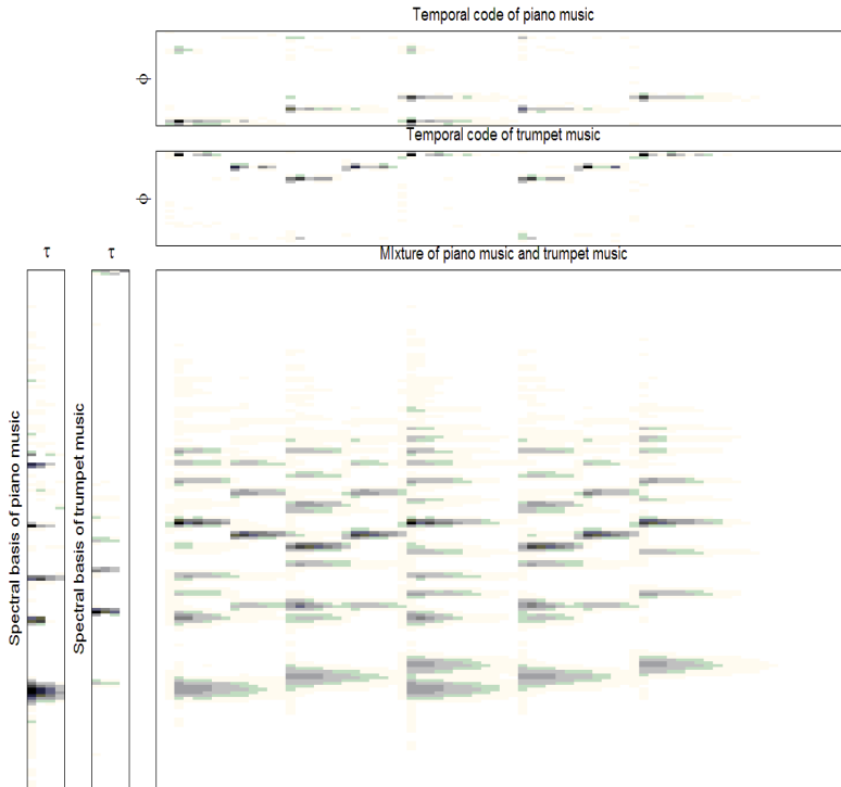
Fig. 1. The estimated spectral dictionary and temporal code of piano and trumpet mixture log-frequency spectrum using SNMF2D.
