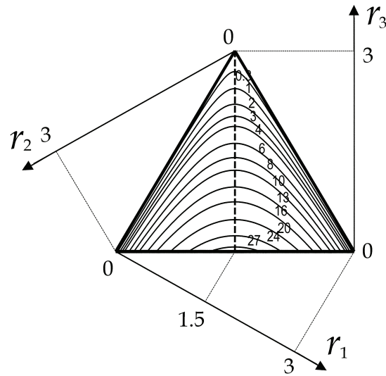
Figure 15. Atlas of the theoretical workspace of the parallel robot
