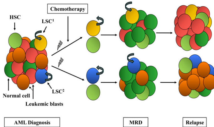
Figure 1. The role of minimal residual disease and leukemic stem cells in the emergence of relapse. HSC, normal hematopoietic stem cell, LSC, leukemic stem cell. At AML diagnosis a heterogeneous population of cells often coexist, including different subpopulations of LSCs. MRD frequency assessment focuses on the detection of leukemic cells present after treatment. Different subpopulations of chemotherapy resistant LSCs can grow out and cause relapse (discussed in section 3).
