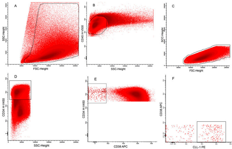
Figure 3. Gating strategy for CD34 + CD38 - LSC detection at diagnosis in AML bone marrow. Gating of viable white blood cells (A). Gating of blast cells with CD45 dim expression and low sideward scatter (SSC) (B, C). CD34 positive progenitors cells (D). Gating of the CD34 positive and CD38 negative blasts (E). The CD34 + CD38 - cells gated against CLL-1. Two populations of stem cells are shown: a CLL-1 negative stem cell population, containing the HSCs and the CD34 + CD38 - cells with positive expression of CLL-1. These stem cells with aberrant expression of CLL-1 are defined as LSCs (F).
