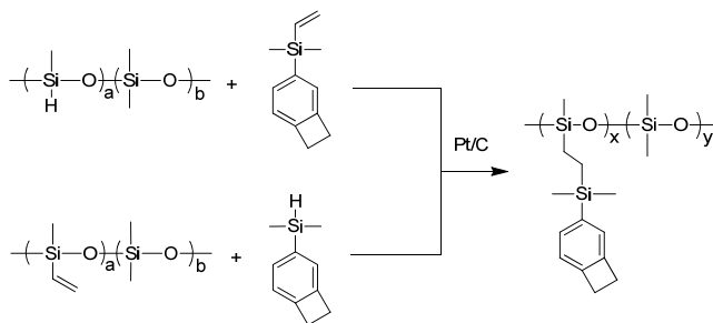
Scheme 10. Preparation of polysiloxane with BCB containing pendant groups.
