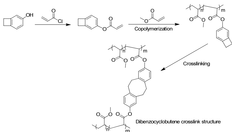
Scheme 6. Preparation and cross-linking of 4-ABCB/MA copolymer.
