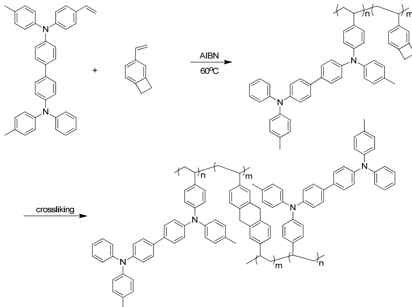
Scheme 14. Preparation and cross-linking of TPD-BCB copolymers.
