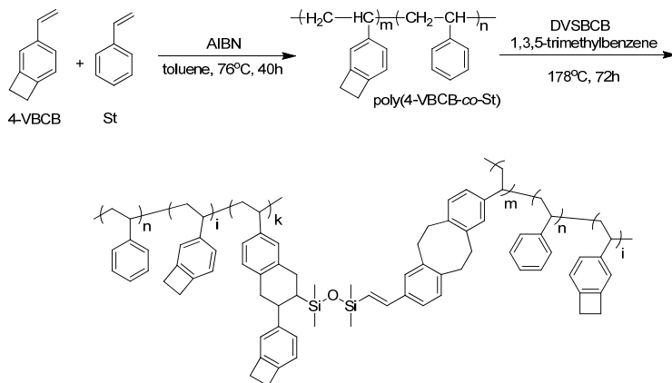
Scheme 8. Preparation of poly(4-VBCB-co-St) and the conetwork structure with DVSBBCB.
