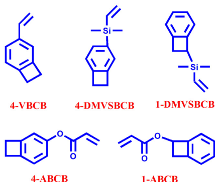
Scheme 3. Chemical structure of several new vinyl-BCBs
