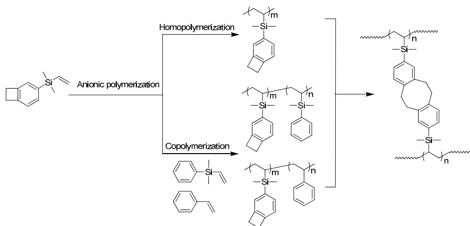
Scheme 4. Anionic homo and copolymerization of 4-DMVSBCB
