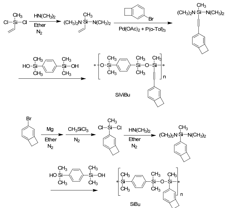
Scheme 11. Synthesis route to copolymers originated from SiViBu and SiBu, respectively.
