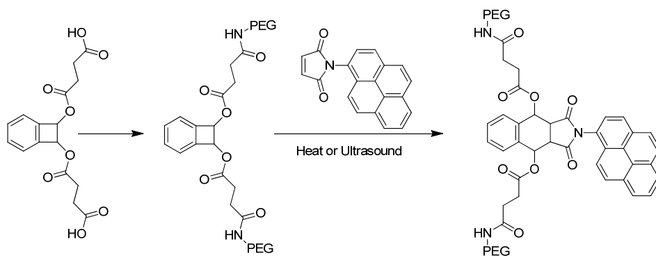
Scheme 15. Preparation and reaction of mechanosensitive polymers.
