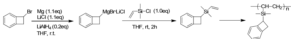
Scheme 5. Synthesis route of 1-DMVSBCB and poly(1-DMVSBCB)
