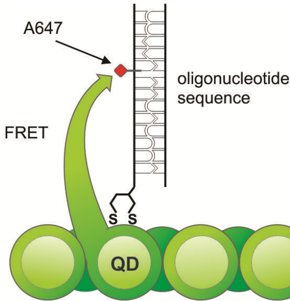
Figure 10. Schematic representation of a FRET process. Immobilized QDs are derivatized with dithiol-terminated probe oligonucleotides and under light excitation the QDs are involved in the emission of the Alexa Fluor 647 dye bound to a determined oligonucleotides sequence (Algar & Krull, 2008; Medintz & Mattoussi, 2009).
