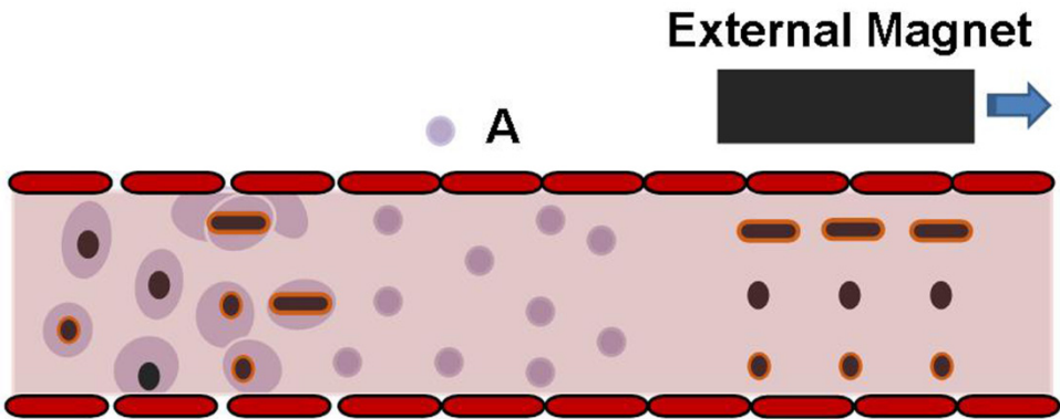
Figure 6. Schematic diagram depicting cell death (A) and excretory organ delivery of nanoparticles under the influence of external magnetic field.
