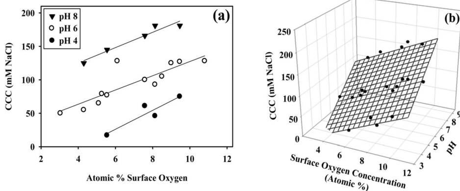
Figure 7. (a) Influence of surface oxygen concentration on the critical coagulation of O-MWNTs at pH = 4, 6 and 8; (b) three dimensional plot showing the functional interdependence of surface oxygen concentration, pH, and CCC of O-MWNTs. (Reprinted with permission from [Smith et al., 2009b]. Copyright, American Chemical Society).
