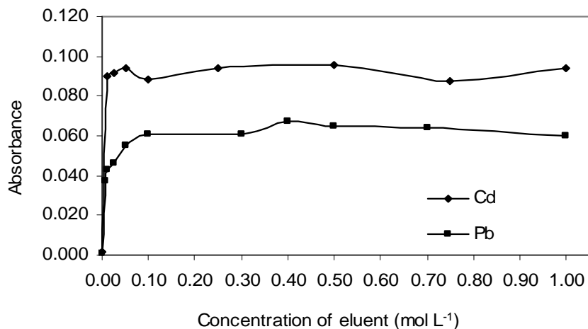
Figure 7. Influence of eluent concentration on the determination of Cd and Pb using solid phase extraction.
