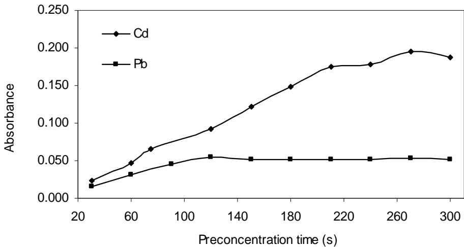
Figure 9. Influence of preconcentration time on the determination of Cd and Pb using solid phase extraction.
