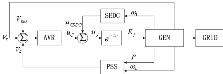
Figure 3. The signal relationship of the SEDC and the excitation regulators (AVR: automatic voltage regulator, PSS: power system stabilizer)
