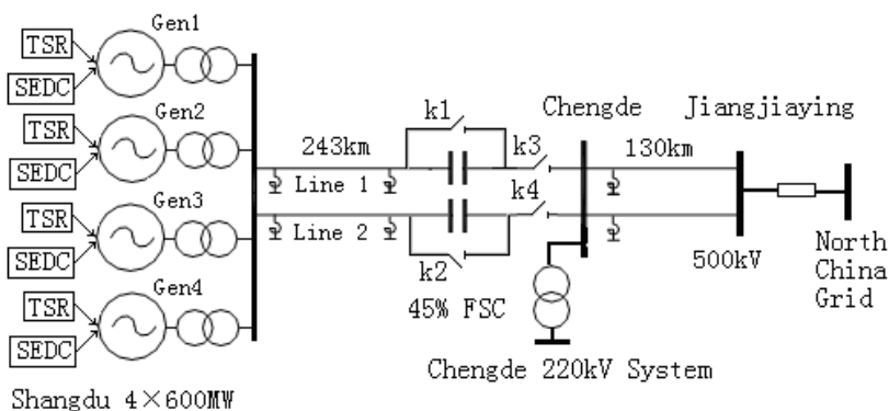
Figure 2. The one-line diagram of the equivalent transmission system
