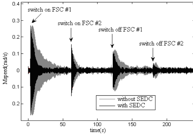
Figure 7. Dynamics of mode 2 during FSCs' switching-on/off operations under the 3-machine condition (unit 4)
