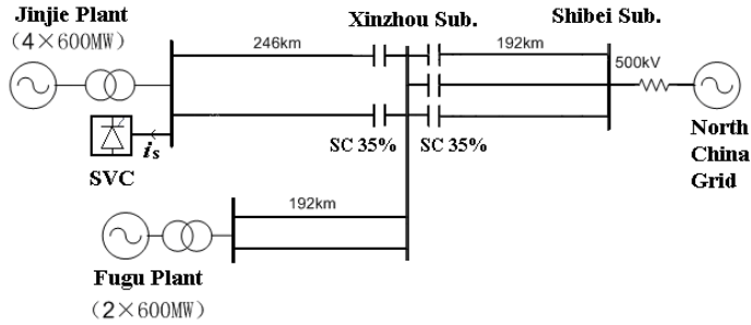
Figure 9. The one-line diagram of the equivalent transmission system
