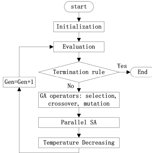
Figure 1. Flow chart of the implemented GA-SA
