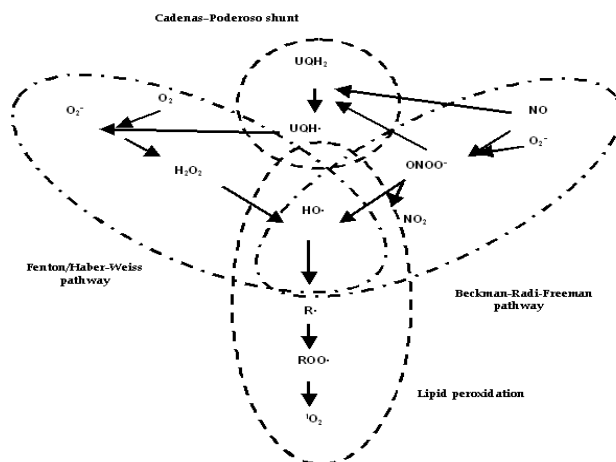
Figure 3. The free-radical mediated chain reaction in biochemistry. O_2^{\cdot-} , superoxide radical; H_2O_2 , hydrogen peroxide; HO\cdot , hydroxyl radical; NO , nitric oxide; ONOO^- , peroxynitrite; \cdot NO_2 , nitrogen dioxide; UQH_2 , ubiquinol; UQH\cdot , ubisemiquinone; R\cdot , alkyl radical; ROO\cdot , peroxy radical; ^1O_2 , singlet oxygen.
