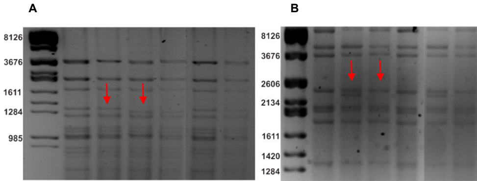
Figure 3. Mitochondrial DNA restriction profiles of T. delbrueckii strains obtained with the (A) Hin I and (B) Hae III restriction endonucleases in 1.5% agarose gel (unpublished results from our laboratory). Lane 1 – Molecular Marker Lambda DNA/Eco47I ( Ava II) from Fermentas; Lane 2 – T. delbrueckii ISA1082 (reference strain); Lane 3 – T. delbrueckii PYCC 5321; Lane 4 – T. delbrueckii PYCC 5323; Lane 5 – 62C; Lane 6 – 45A; Lane 7 – 45D. Arrows indicate main differences between profiles I and II. Yeast cells were cultivated in 1 ml YPD (1% yeast extract, 2% peptone, 2% glucose) for 24 h at 30 °C and 160 r.p.m and DNA isolation was performed as previously described (126). Digestion was carried out with Hin I or Hae III restriction enzymes overnight at 37 °C, in a final volume of 20 \mu l as previously described (123). Restriction fragments were separated in horizontal 1.5% agarose gels run in 0.5X TBE buffer at 60 V for six hours and visualized in a UV transilluminator (Eagleeye II Image Acquisition System, Stratagene, La Jolla, CA) after ethidium bromide staining.
