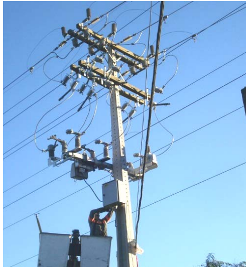
Fig. 8. Installation of a remote controlled switch.
