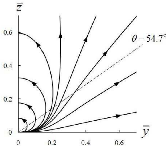
Fig. 10. The figure shows field lines of the Poynting vector for a dipole oscillating along the z axis and embedded in a material with \epsilon_r = 1.7 + 0.06i and \mu_r = 1 . These are the values for water at 3 \mu\text{m} . The index of refraction is n = 1.3 + 0.023i .
