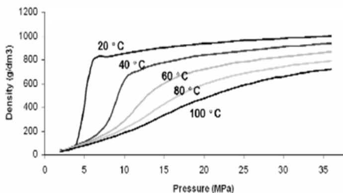
Fig. 4. The density of \text{CO}_2 as a function of pressure for a range of temperatures
