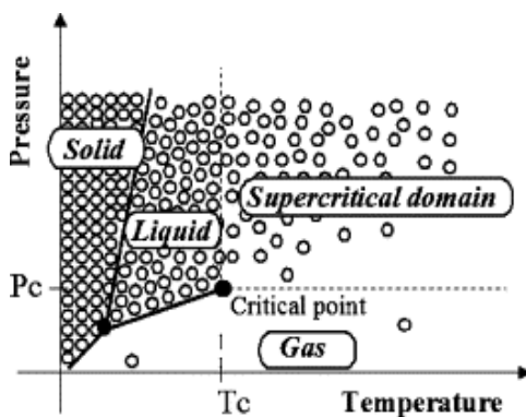
Fig. 3. A schematic representation of the microscopic behaviour of a pure fluid in the P-T plane phase diagram (Cansell et al., 2003)
