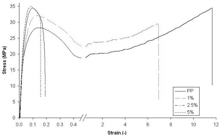
Fig. 9. Stress-strain curves of scCO 2 PP / sepiolite nanocomposites with different clay contents (Ma et al., 2007)
