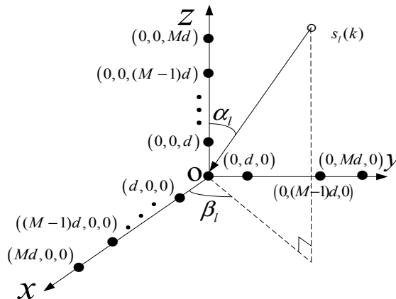
Fig. 16. Two L-shape array configuration
