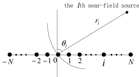
Fig. 6. Uniform linear array configuration
