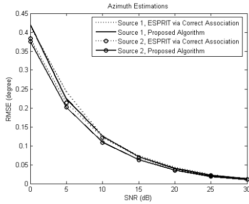
Fig. 3. RMSE of azimuth angle estimations versus SNR
