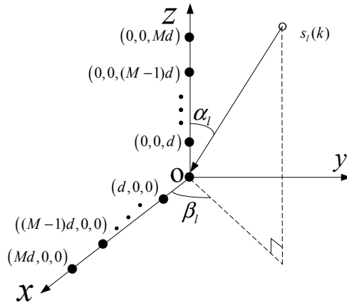
Fig. 1. L-shaped sensor array configuration
