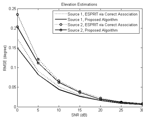
Fig. 2. RMSE of elevation angle estimations versus SNR
