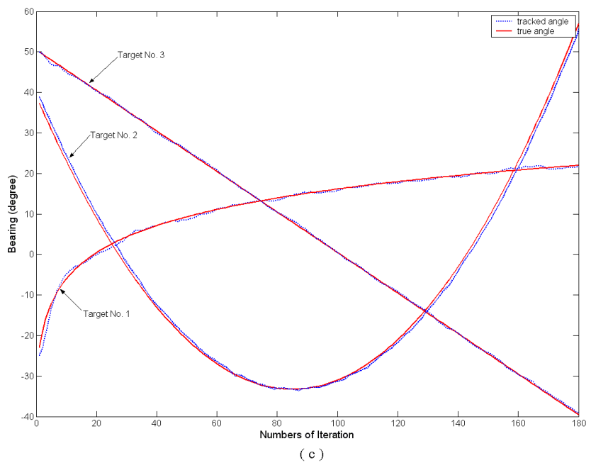
Fig. 3. Typical sample run for crossing tracks with three targets at SNR=10dB. (a) Kong's algorithm, (b) Park's algorithm, (c) PAT-EKF algorithm
