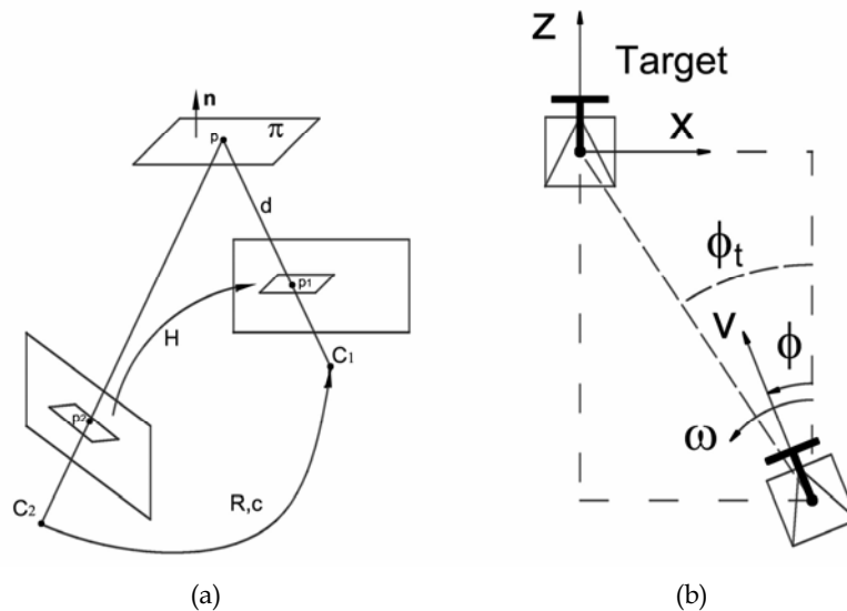
Figure 1. (a) Homography from a plane between two views. (b) Coordinate system
